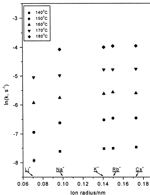
Figure 10. Effect of the Group 1 cations on the decarboxylation rate of HCCCO 2 - at various temperatures.
