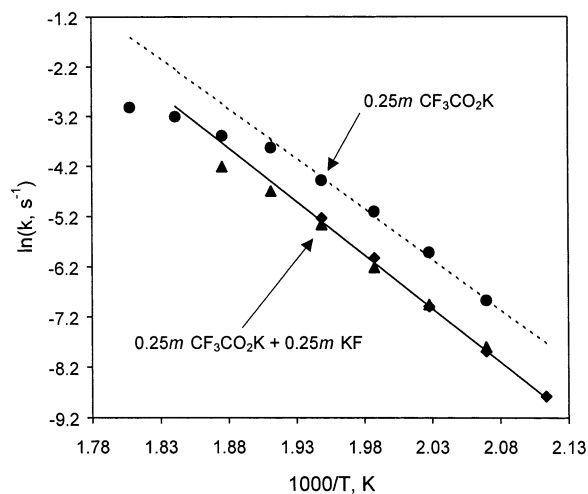
Figure 6. Arrhenius plot showing that the addition of 0.25 m KF to 0.25 m K[CF 3 CO 2 ] slows down the decarboxylation rate. The dashed line fits the four lowest temperature data points to emphasize the curvature at the higher temperatures.
